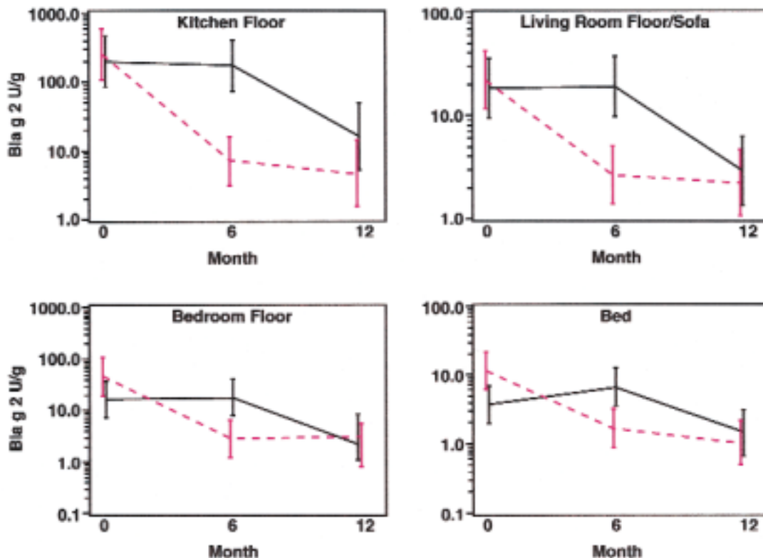
FIG 2. Geometric mean Bla g 2 allergen concentrations (and 95% confidence intervals) from vacuumed dust samples in control (solid black lines) and intervention (dashed red lines) homes. Control homes received no interventions from months 0 to 6 and insecticide application at months 6 and 9.
