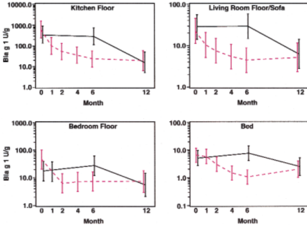
FIG 1. Geometric mean Bla g 1 allergen concentrations (and 95% confidence intervals) from vacuumed dust samples in control (solid black lines) and intervention (dashed red lines) homes. Control homes received no interventions from months 0 to 6 and insecticide bait application at months 6 and 9.
